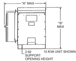
Dimensions Three-Phase
